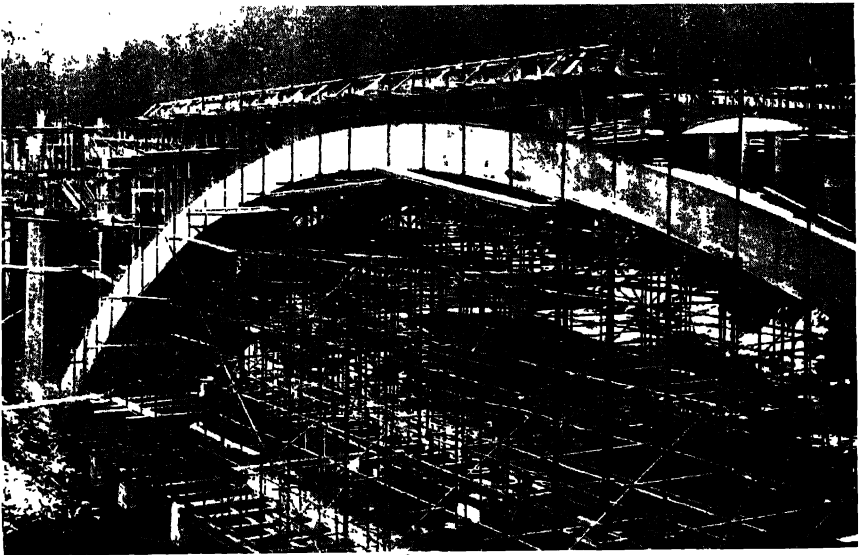
Fig. 283. Arch Staging supported on River Bed.
